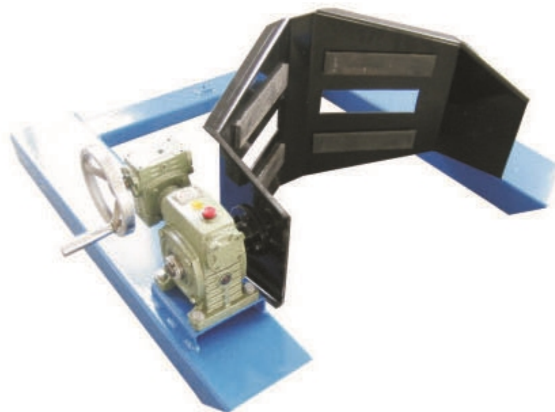
HK285E欧式搬运夹 (蜗轮翻转多功能) (worm gear flipping & multifunctional)
